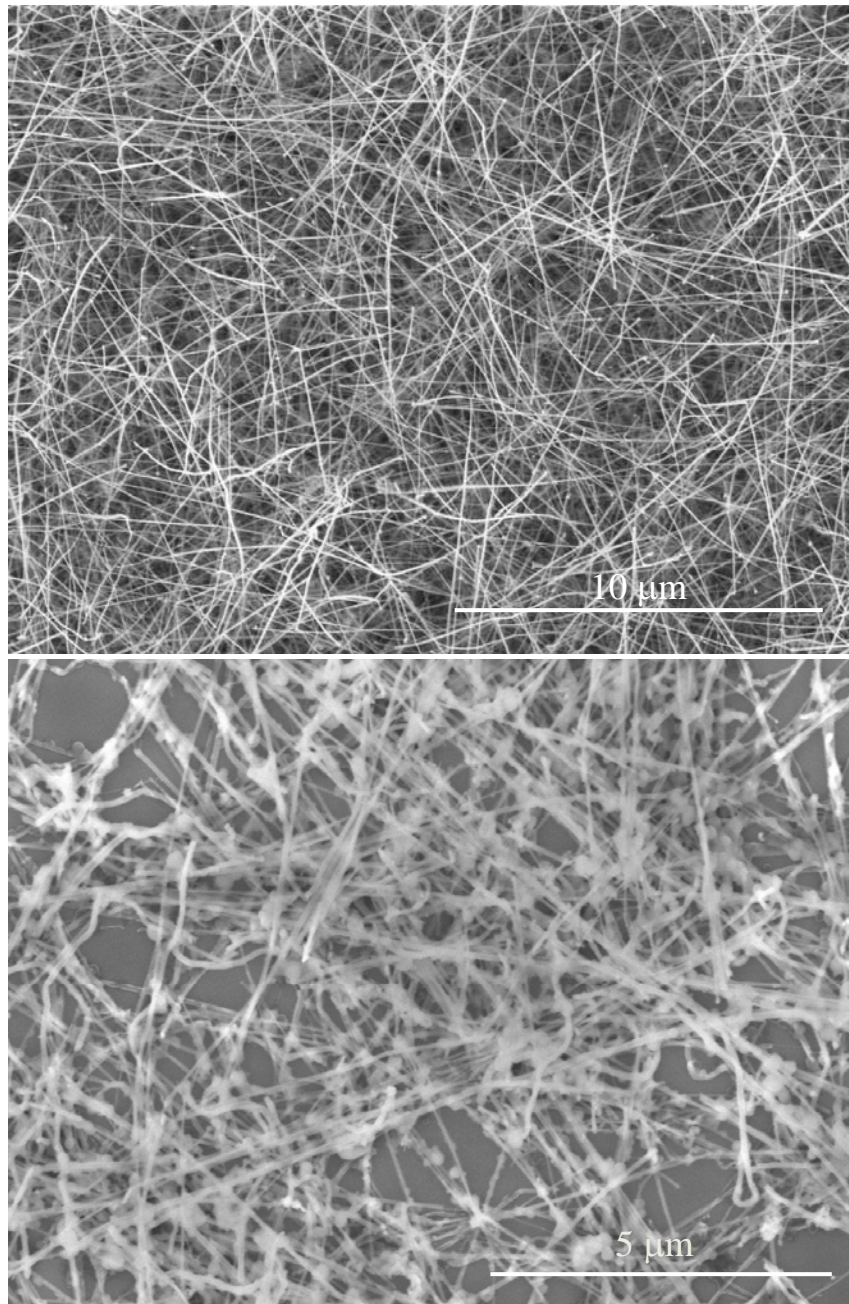
Figure S3. SEM image of as grown BNNTs dispersed in ethanol spin coated on silica substrate (upper picture), and SEM image of composite membrane of BNNTs and polymer A which was spin coated on silica substrate (lower picture).
