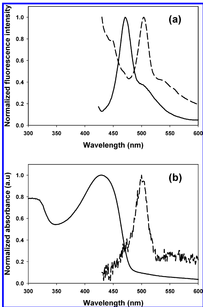
FIGURE 5. (a) Fluorescence spectra of polymer B (dark line) and its composite material with BNNTs (dashed line) in \text{CHCl}_3 , (b) absorption spectrum of polymer B (dark line), corrected spectrum of composite material of BNNTs and polymer B (dash line) in \text{CHCl}_3 .
