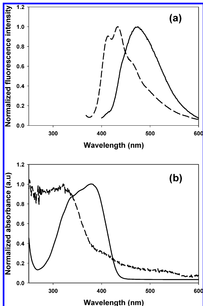
FIGURE 6. (a) Fluorescence emission spectra of polymer C (dark line) and its composite with BNNTs (dashed line) in \text{CHCl}_3 , (b) Absorption spectrum of polymer C (dark line), corrected spectrum of composite material of BNNTs and polymer C (dash line) in \text{CHCl}_3 .
