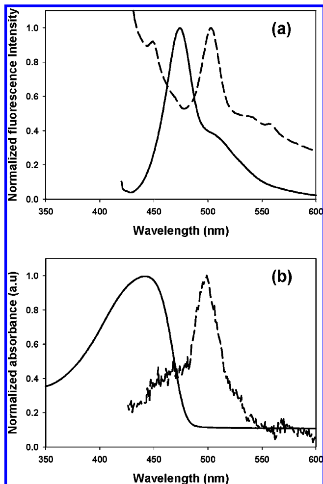
FIGURE 3. (a) Fluorescence spectra of polymer A (dark line) and composite of BNNTs and polymer A in \text{CHCl}_3 (dashed line), (b) absorption spectrum of polymer A (dark line), and corrected absorption spectrum of composite of BNNTs and polymer A (dashed line) in \text{CHCl}_3 .
