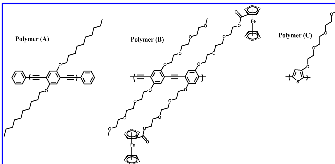
Scheme 1. Chemical Structures of PPEs (Polymers A and B) and Regioregular Head-to-Tail Polythiophene (Polymer C)
